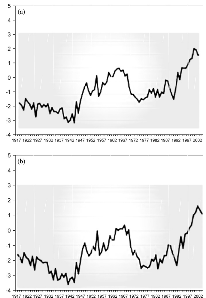
Fig. 1. Warming index in Córdoba (a) and Granada (b) from 1917 to 2005.
