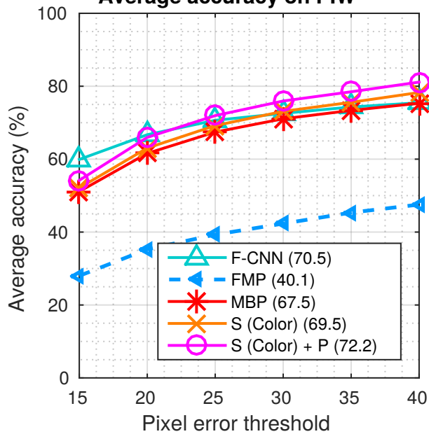
Average accuracy on PIW
