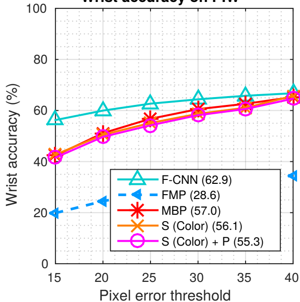
Wrist accuracy on PIW
