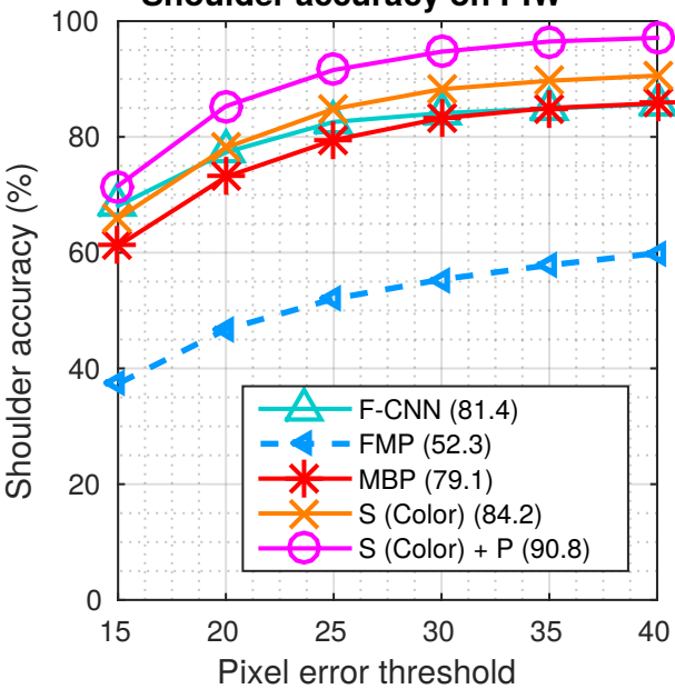
Shoulder accuracy on PIW
