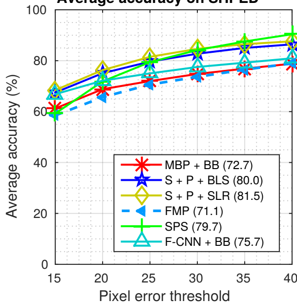
Average accuracy on SHPED
