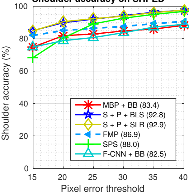
Shoulder accuracy on SHPED
