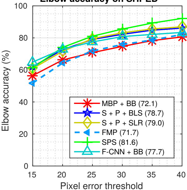
Elbow accuracy on SHPED
