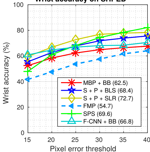
Wrist accuracy on SHPED
